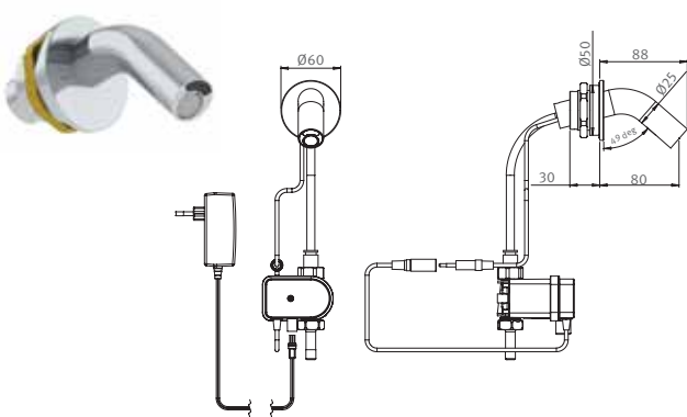
EXTREME FW Exposed installation 237709 EXTREME FW , 9V Transformer
