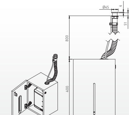
• 07220090CB Top-Filling Multifeed With lockable cabinet
