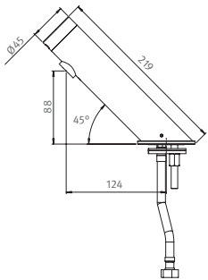
GREEN AB1953 • 225901 GREEN AB1953, Internal 9V Battery
