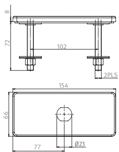
07270288 COVER PLATE 4" ANTI-ROTATION KIT FOR CSABA
