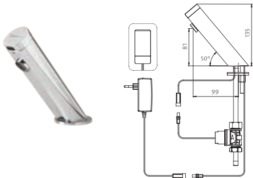
TOUCH FREE AB1953 • 225610 TOUCH FREE B AB1953, 9V Battery • 225710 TOUCH FREE E AB1953, 9V Transformer
