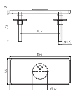
07270291 COVER PLATE 4" ANTI-ROTATION KIT FOR TRENDY/EXTREME
