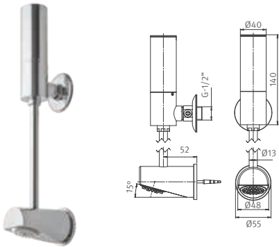
FOOT WASHFREE Exposed installation 113730 FOOT WASHFREE , Internal 9V battery
