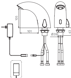
SWAN 1000 B/E AB1953 Mixer to adjust water temperature • 252310 SWAN 1000 B AB1953, 9V Battery • 252420 SWAN 1000 E AB1953, 9V Transformer
