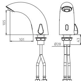
SWAN 1000 AB1953 Mixer to adjust water temperature • 252210 SWAN 1000 AB1953, Internal 9V Battery
