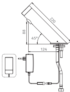
GREEN B/E AB1953 • 225951 GREEN B AB1953, 9V Battery • 225941 GREEN E AB1953, 9V Transformer
