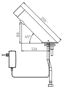
GREEN BRE AB1953 Features a permanent ring illumination When a user places his hands within the sensor range, the ring of light blinks while water flows from the faucet. • 225921 GREEN BRE AB1953, 9V Transformer
