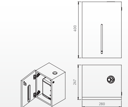
• 07220096CB Below Deck Multifeed Kit With lockable cabinet
