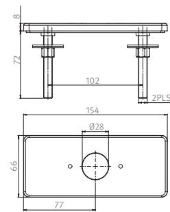
07270290 COVER PLATE 4" ANTI-ROTATION KIT FOR CLASSIC CS
