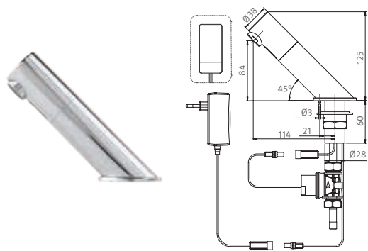
TUBULAR DM • 350700 TUBULAR DMB, 9V Battery • 350750 TUBULAR DME, 9V Transformer
