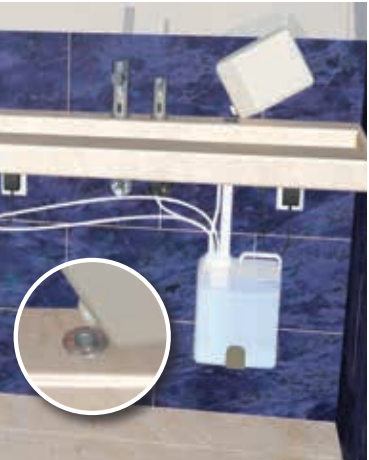
• 07220152 Top-Filling Multifeed Kit with Soap Level Indicator
