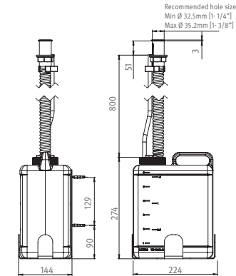
• 07220152 Top-Filling Multifeed Kit with Soap Level Indicator
